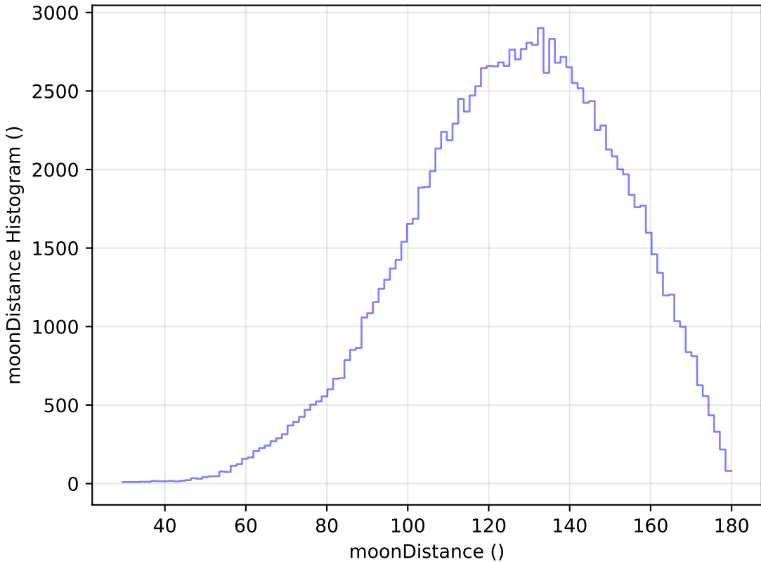
retro_baseline_v2.0_10yrs WFD u band: moonDistance Histogram
