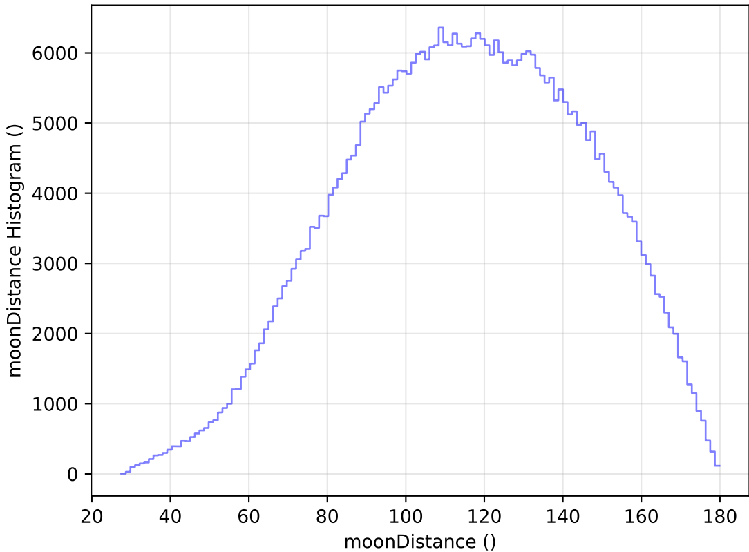
retro_baseline_v2.0_10yrs WFD r band: moonDistance Histogram
