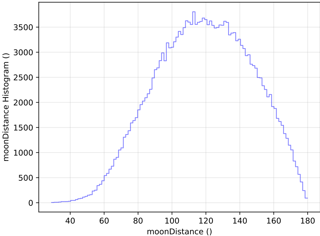
retro_baseline_v2.0_10yrs WFD g band: moonDistance Histogram
