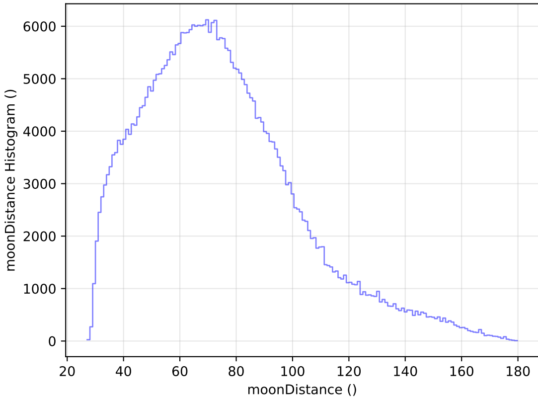
retro_baseline_v2.0_10yrs All sky z band: moonDistance Histogram
