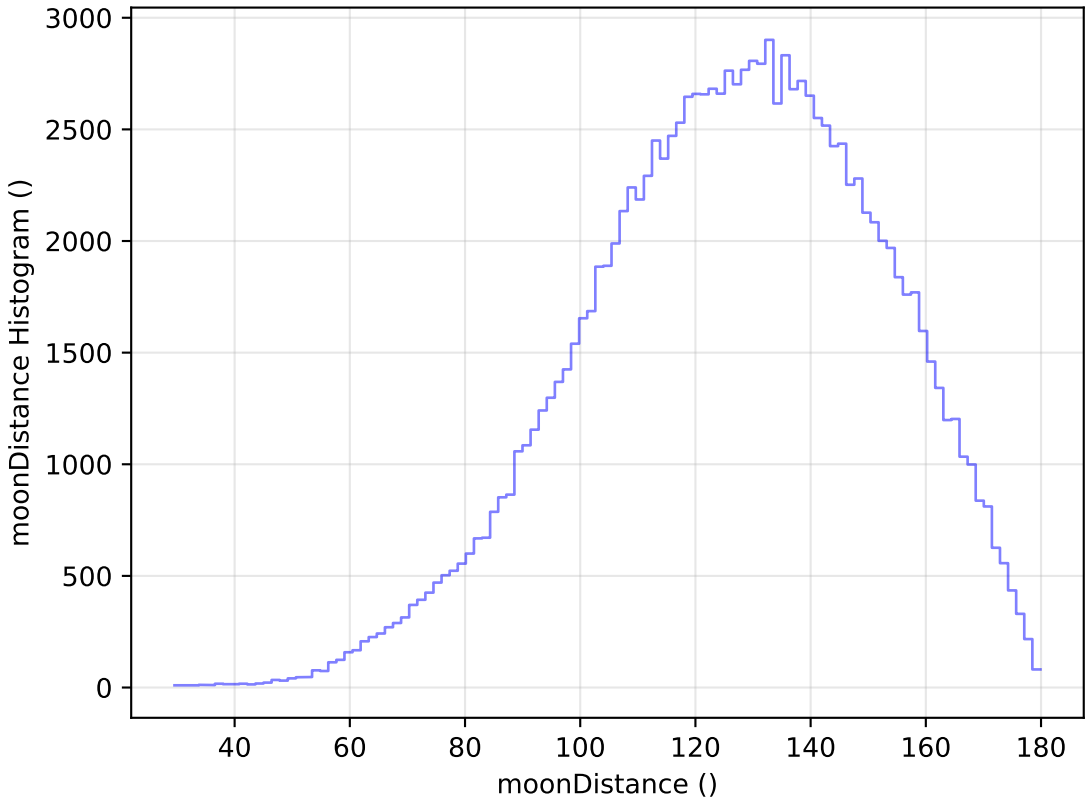
retro_baseline_v2.0_10yrs All sky u band: moonDistance Histogram
