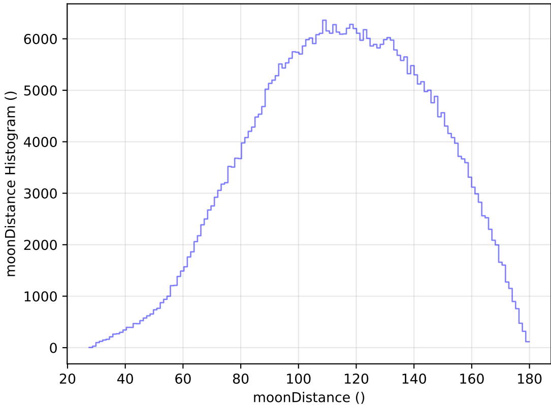
retro_baseline_v2.0_10yrs All sky r band: moonDistance Histogram
