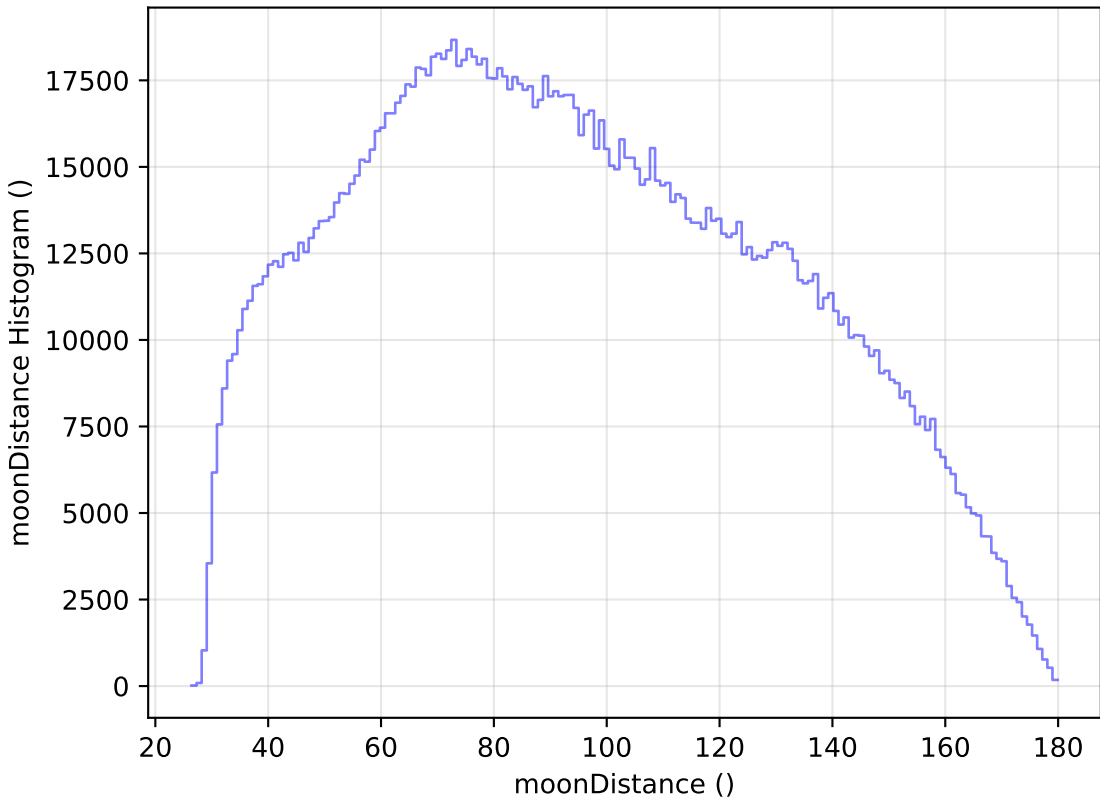
retro_baseline_v2.0_10yrs All sky all bands: moonDistance Histogram
