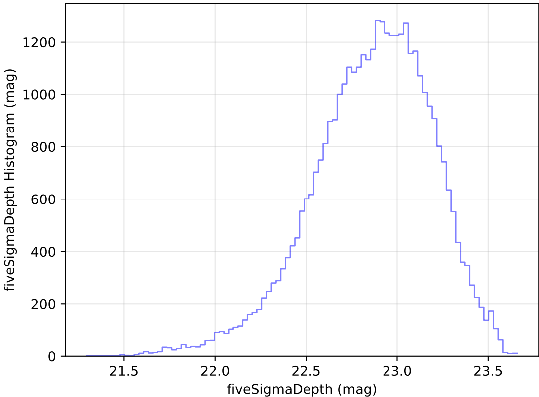
retro_baseline_v2.0_10yrs Yr 1 z band: fiveSigmaDepth Histogram
