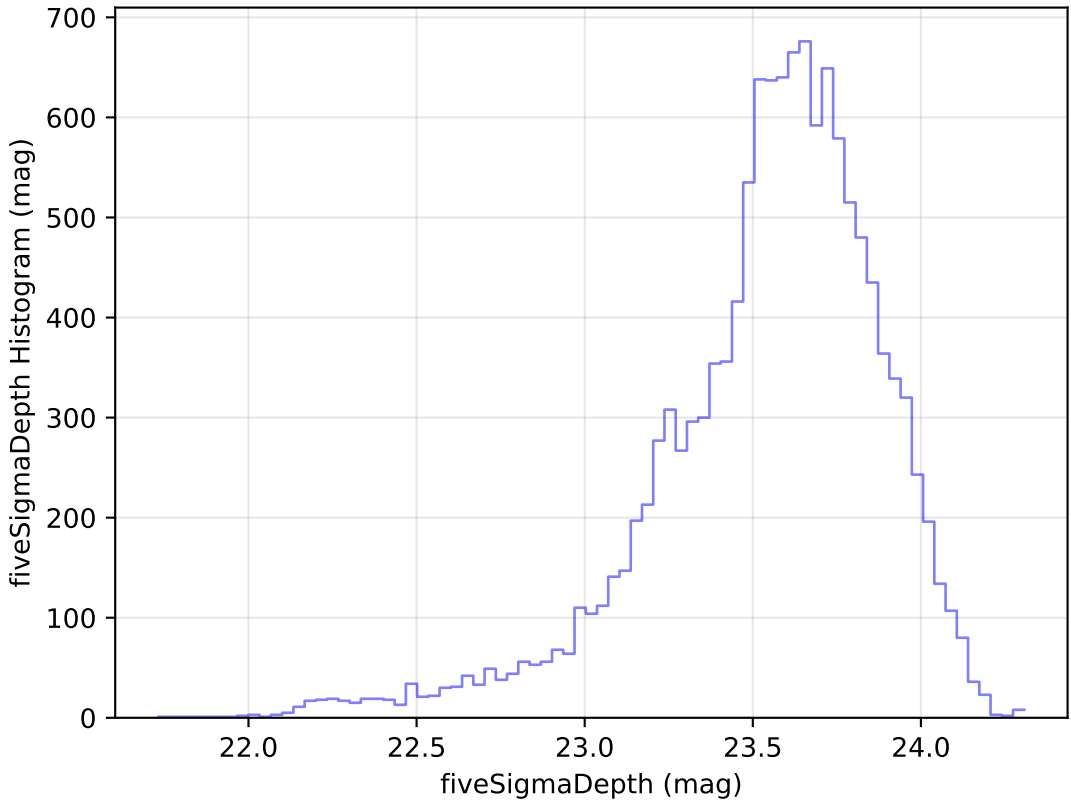
retro_baseline_v2.0_10yrs Yr 1 u band: fiveSigmaDepth Histogram
