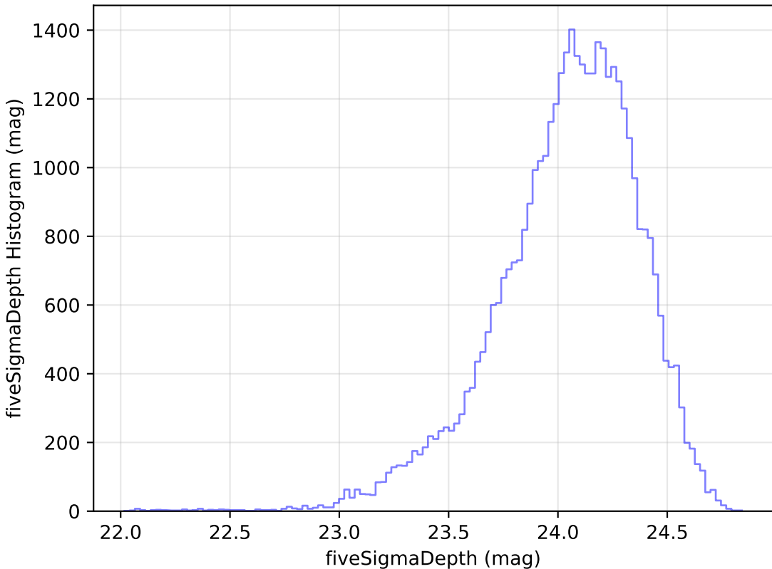
retro_baseline_v2.0_10yrs Yr 1 r band: fiveSigmaDepth Histogram
