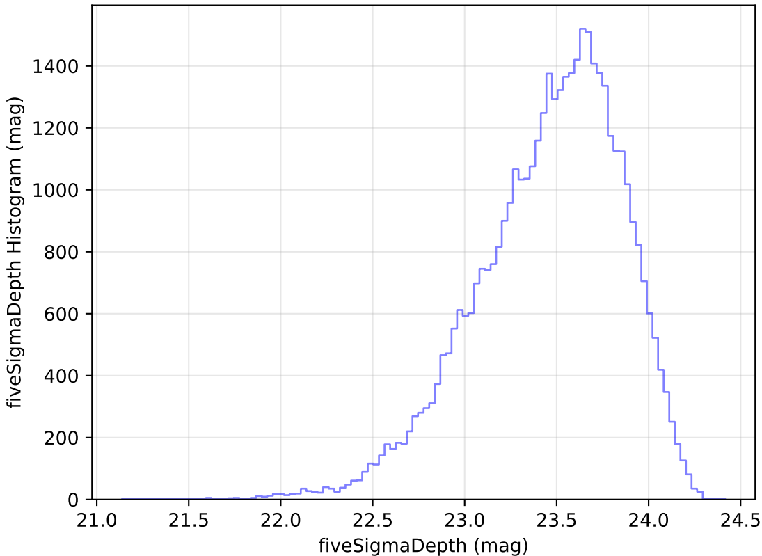
retro_baseline_v2.0_10yrs Yr 1 i band: fiveSigmaDepth Histogram
