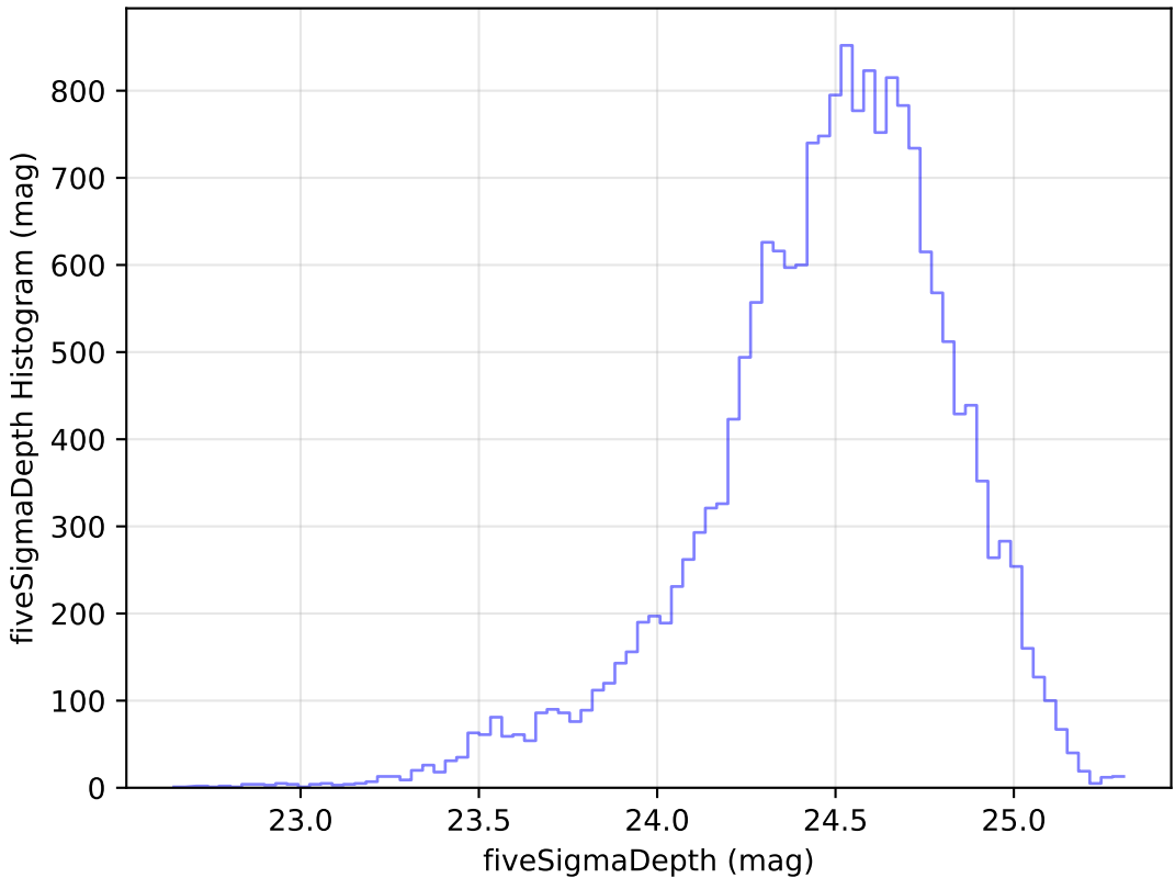
retro_baseline_v2.0_10yrs Yr 1 g band: fiveSigmaDepth Histogram
