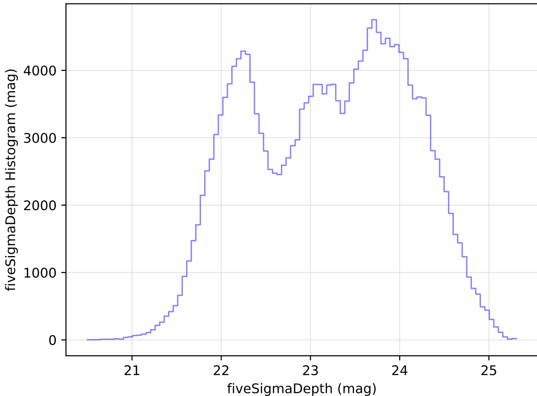
retro_baseline_v2.0_10yrs Yr 1 all bands: fiveSigmaDepth Histogram
