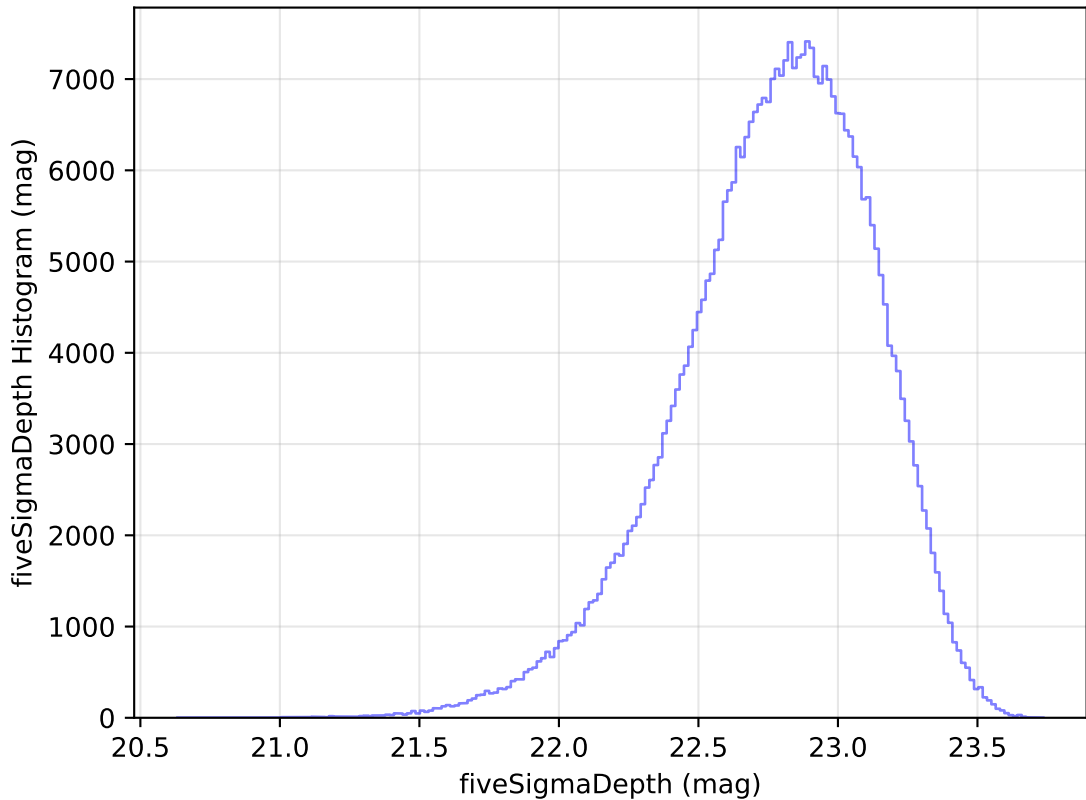
retro_baseline_v2.0_10yrs WFD z band: fiveSigmaDepth Histogram
