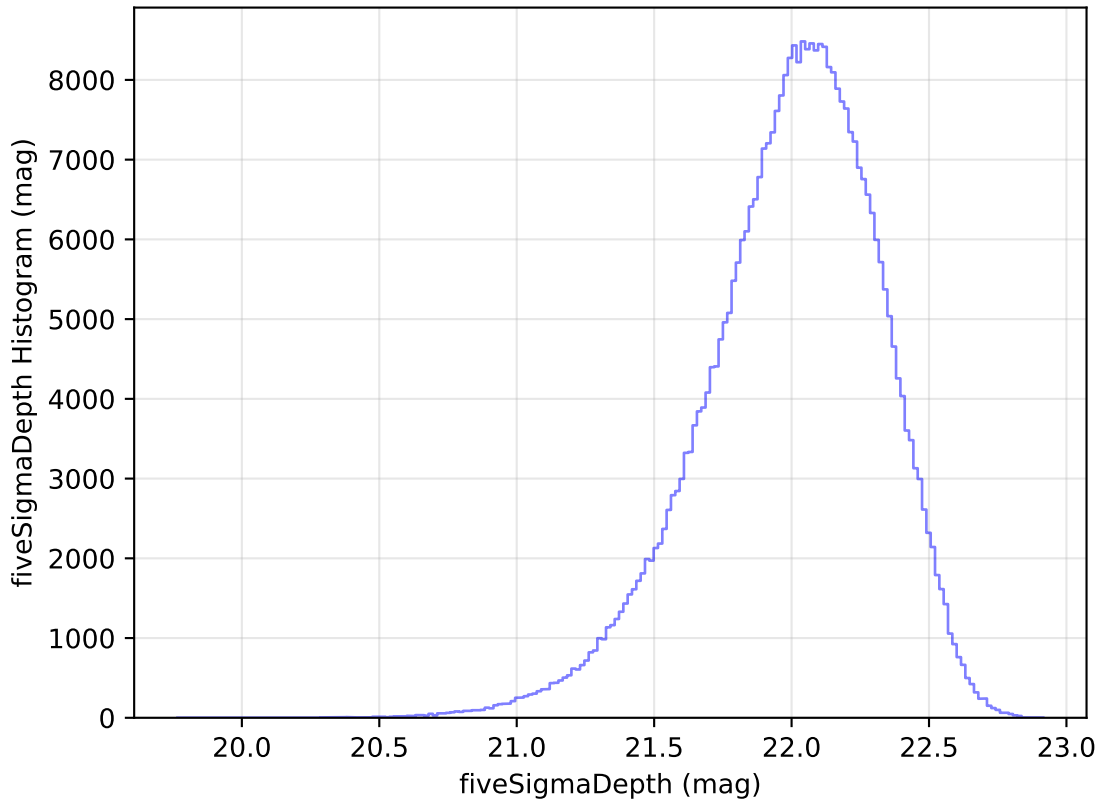
retro_baseline_v2.0_10yrs WFD y band: fiveSigmaDepth Histogram
