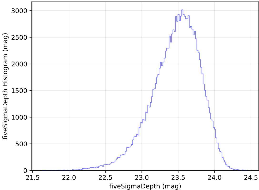
retro_baseline_v2.0_10yrs WFD u band: fiveSigmaDepth Histogram
