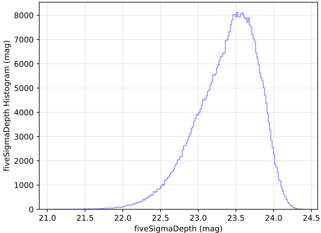
retro_baseline_v2.0_10yrs WFD i band: fiveSigmaDepth Histogram
