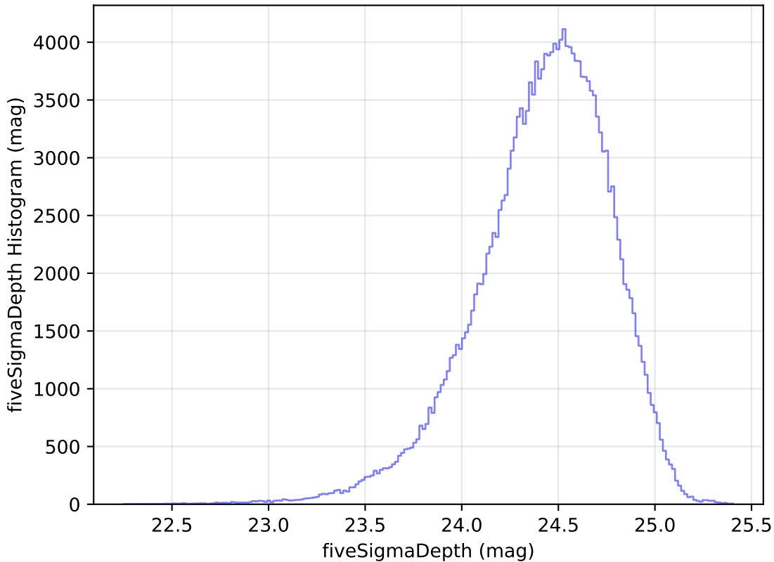
retro_baseline_v2.0_10yrs WFD g band: fiveSigmaDepth Histogram
