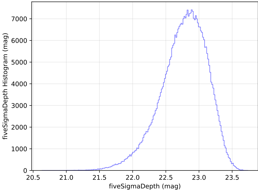
retro_baseline_v2.0_10yrs All sky z band: fiveSigmaDepth Histogram
