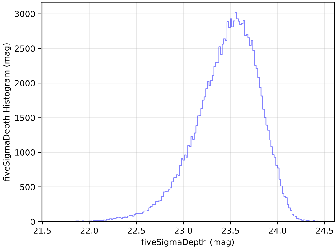
retro_baseline_v2.0_10yrs All sky u band: fiveSigmaDepth Histogram
