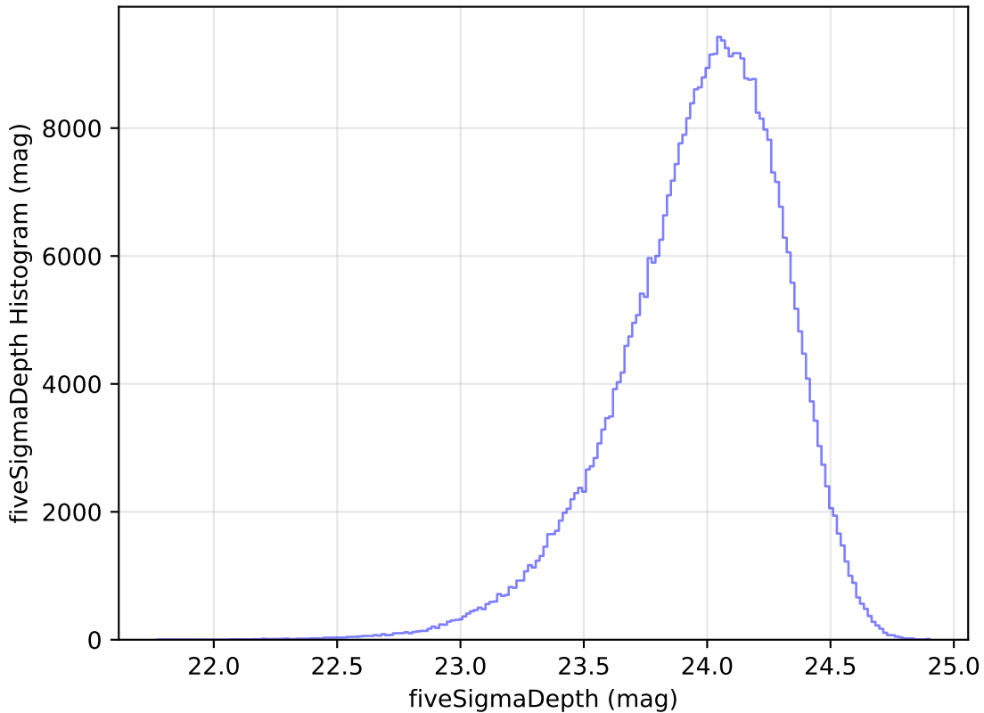
retro_baseline_v2.0_10yrs All sky r band: fiveSigmaDepth Histogram
