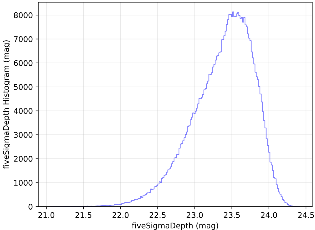
retro_baseline_v2.0_10yrs All sky i band: fiveSigmaDepth Histogram
