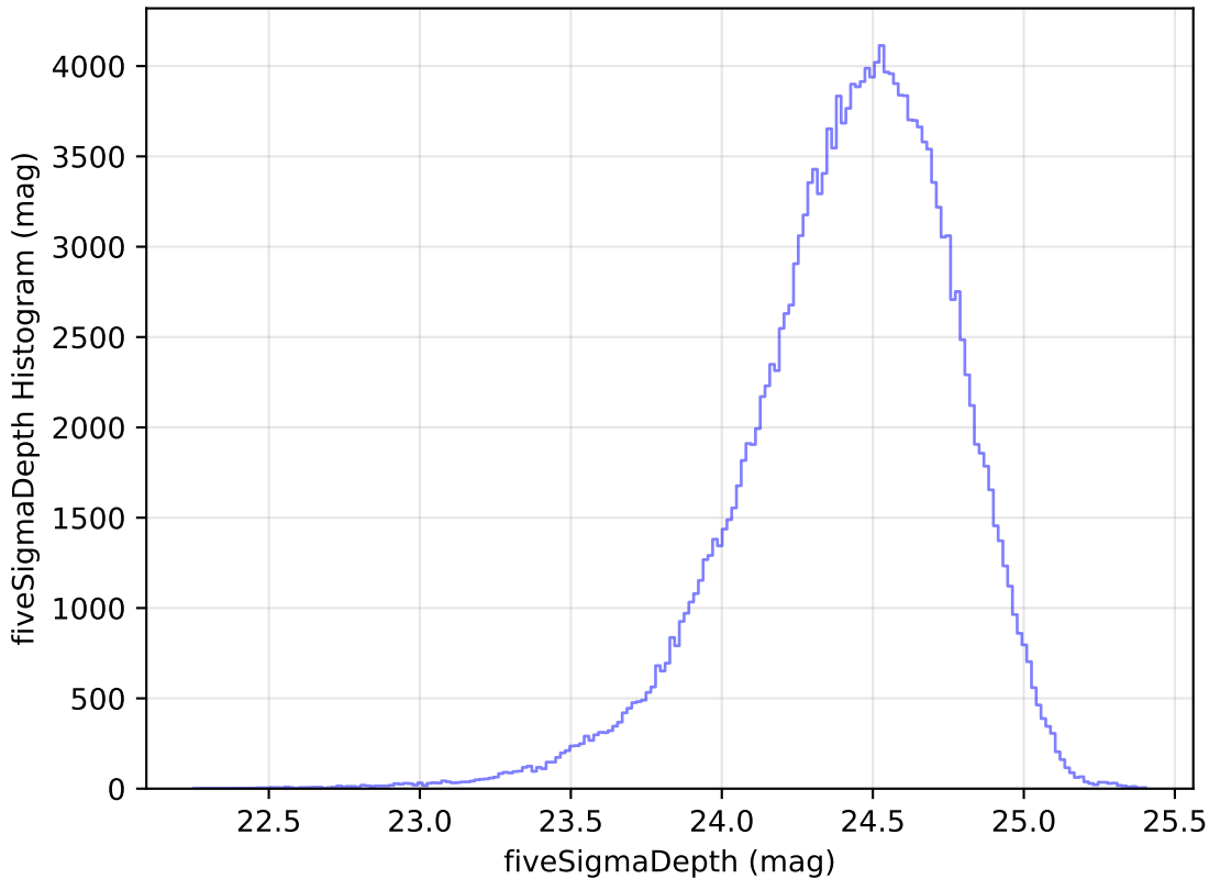
retro_baseline_v2.0_10yrs All sky g band: fiveSigmaDepth Histogram
