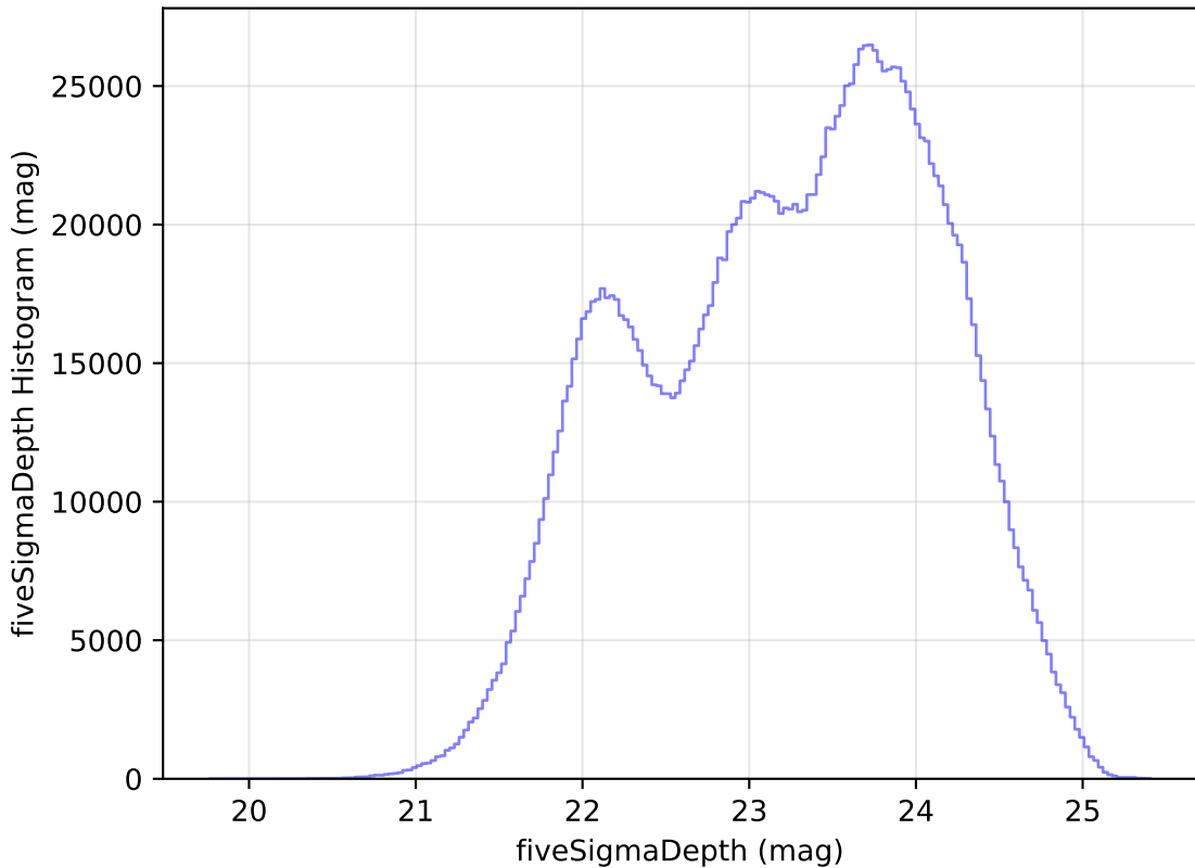
retro_baseline_v2.0_10yrs All sky all bands: fiveSigmaDepth Histogram
