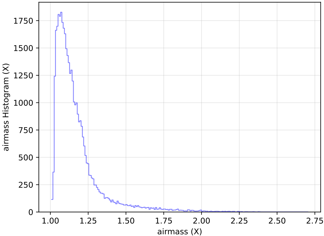
retro_baseline_v2.0_10yrs Yr 1 z band: airmass Histogram
