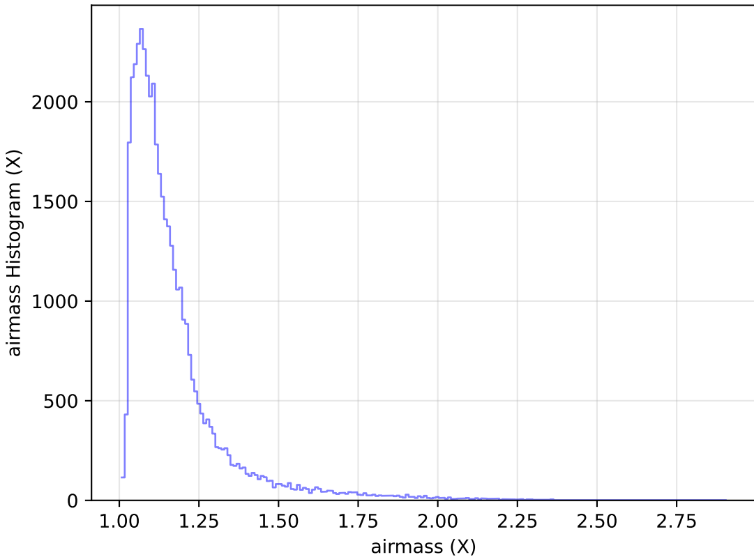
retro_baseline_v2.0_10yrs Yr 1 i band: airmass Histogram
