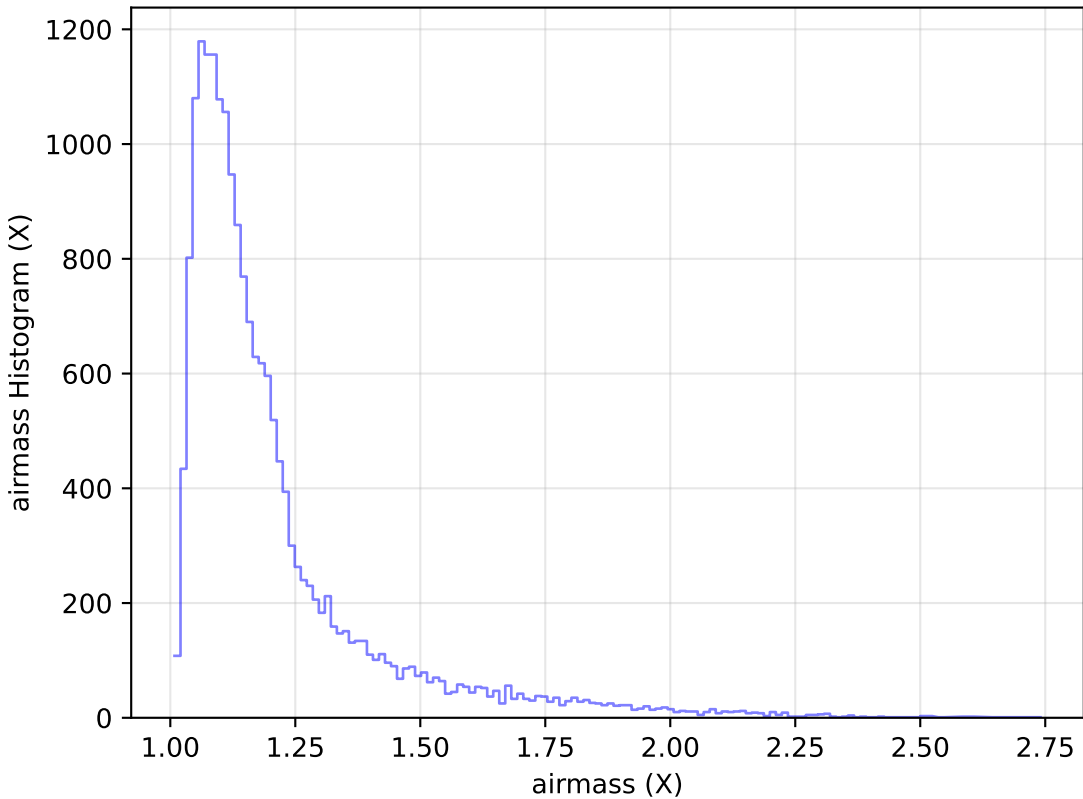
retro_baseline_v2.0_10yrs Yr 1 g band: airmass Histogram
