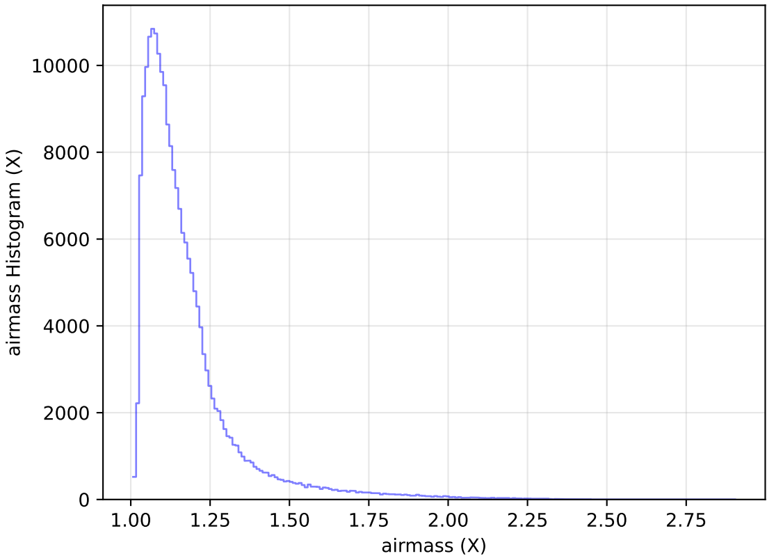
retro_baseline_v2.0_10yrs Yr 1 all bands: airmass Histogram
