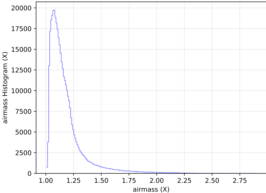
retro_baseline_v2.0_10yrs WFD z band: airmass Histogram
