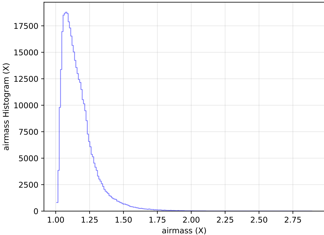
retro_baseline_v2.0_10yrs WFD y band: airmass Histogram
