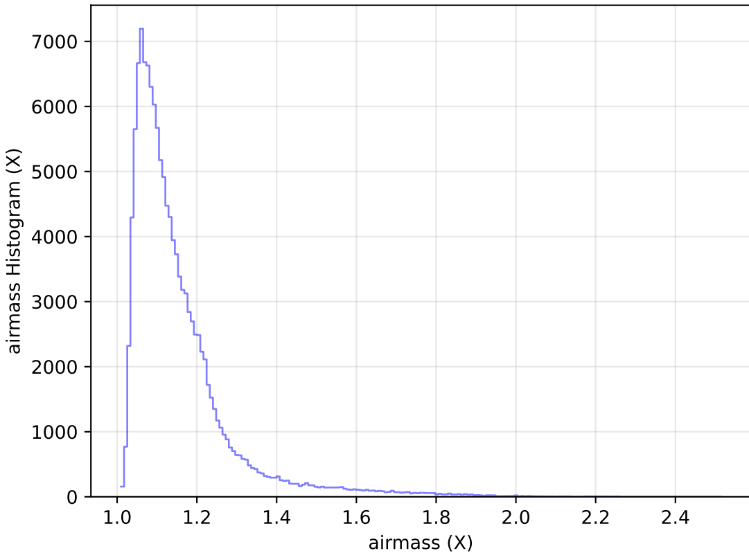
retro_baseline_v2.0_10yrs WFD u band: airmass Histogram
