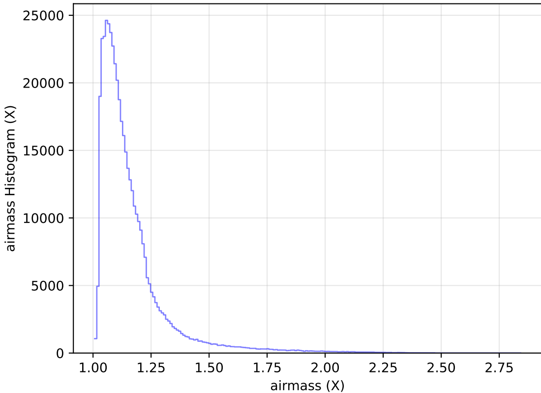
retro_baseline_v2.0_10yrs WFD r band: airmass Histogram
