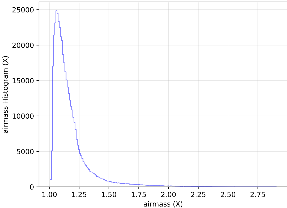
retro_baseline_v2.0_10yrs WFD i band: airmass Histogram
