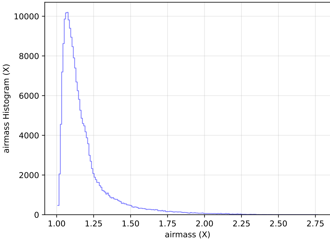
retro_baseline_v2.0_10yrs WFD g band: airmass Histogram
