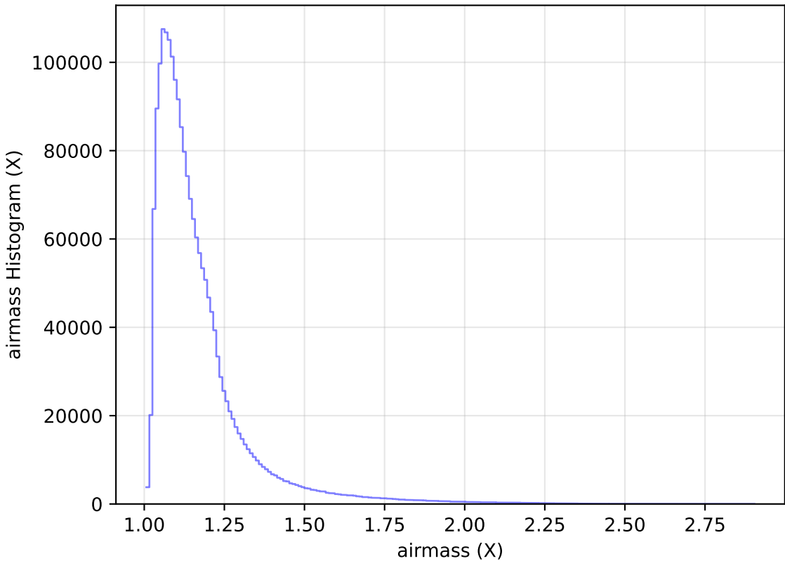
retro_baseline_v2.0_10yrs WFD all bands: airmass Histogram
