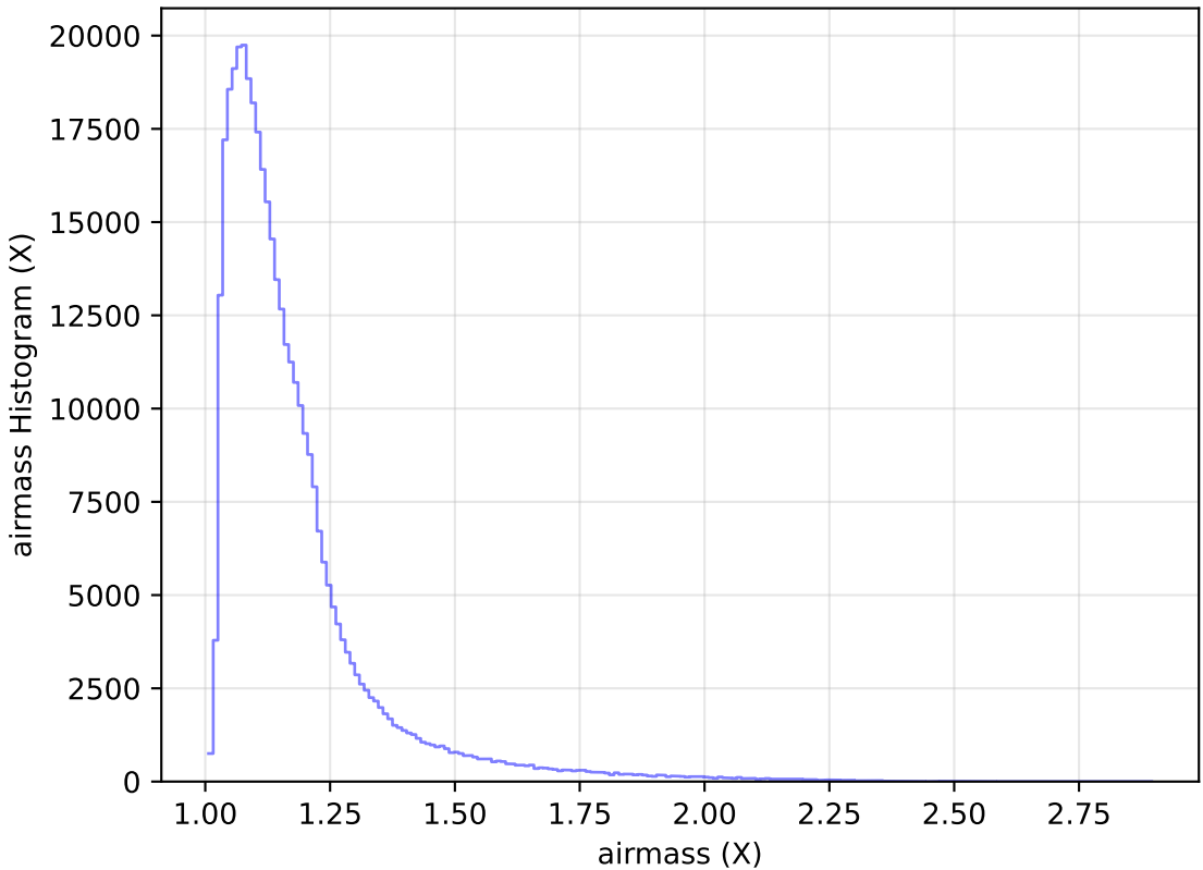
retro_baseline_v2.0_10yrs All sky z band: airmass Histogram
