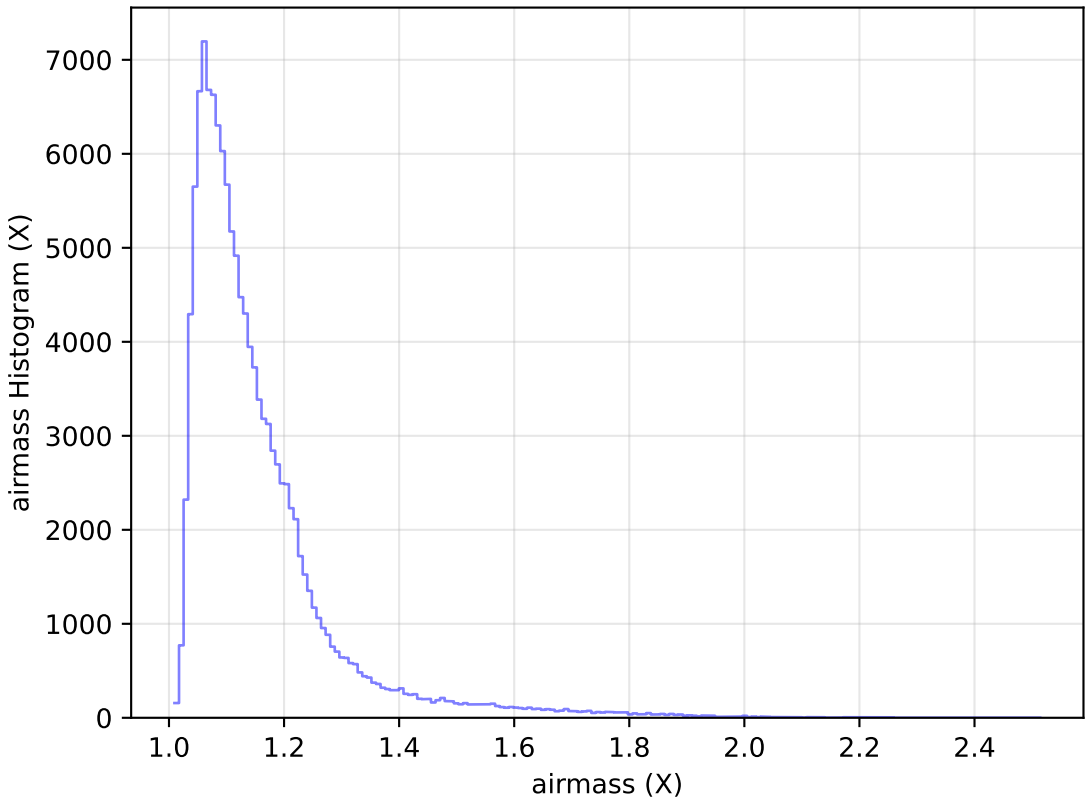
retro_baseline_v2.0_10yrs All sky u band: airmass Histogram
