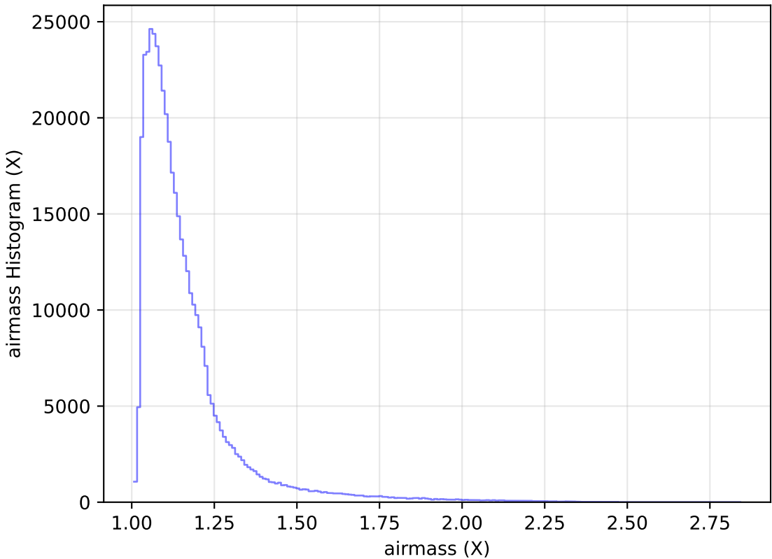
retro_baseline_v2.0_10yrs All sky r band: airmass Histogram
