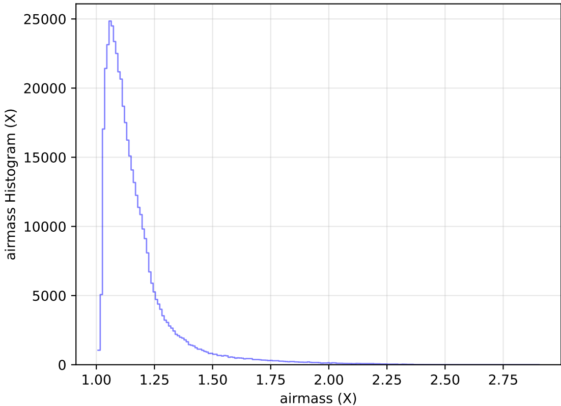
retro_baseline_v2.0_10yrs All sky i band: airmass Histogram
