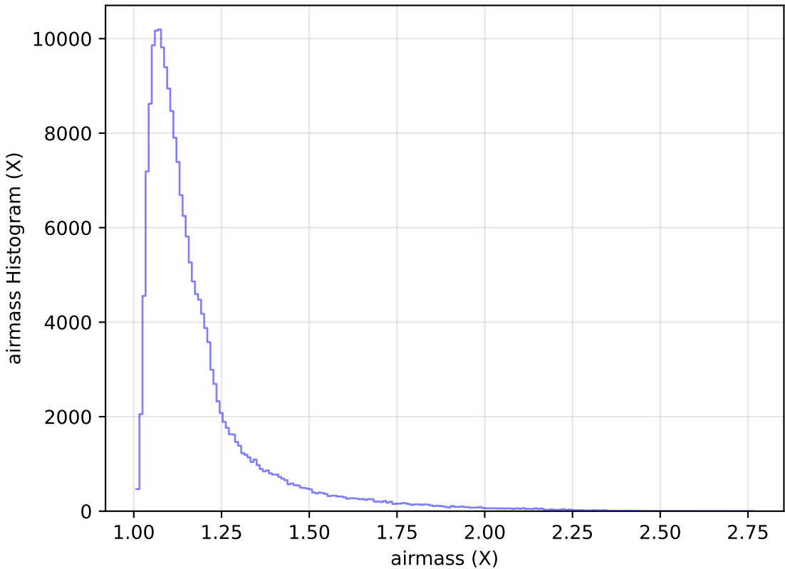
retro_baseline_v2.0_10yrs All sky g band: airmass Histogram
