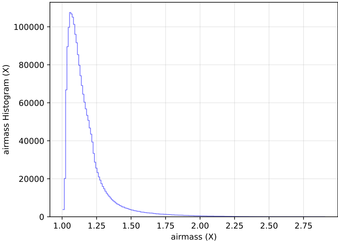
retro_baseline_v2.0_10yrs All sky all bands: airmass Histogram
