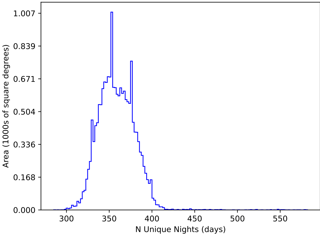
retro_baseline_v2.0_10yrs WFD all bands: N Unique Nights
