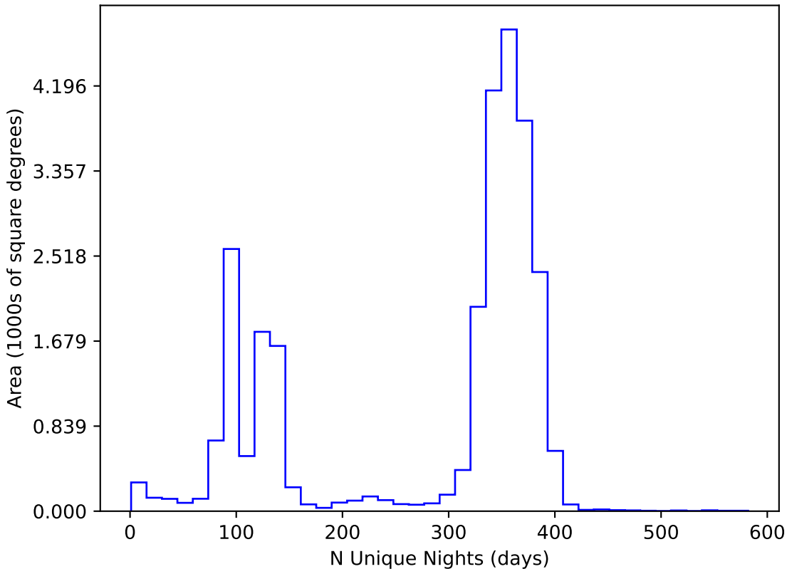
retro_baseline_v2.0_10yrs All sky all bands: N Unique Nights
