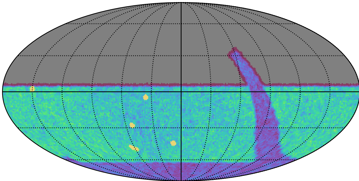
retro_baseline_v2.0_10yrs All sky u band: NVisits
