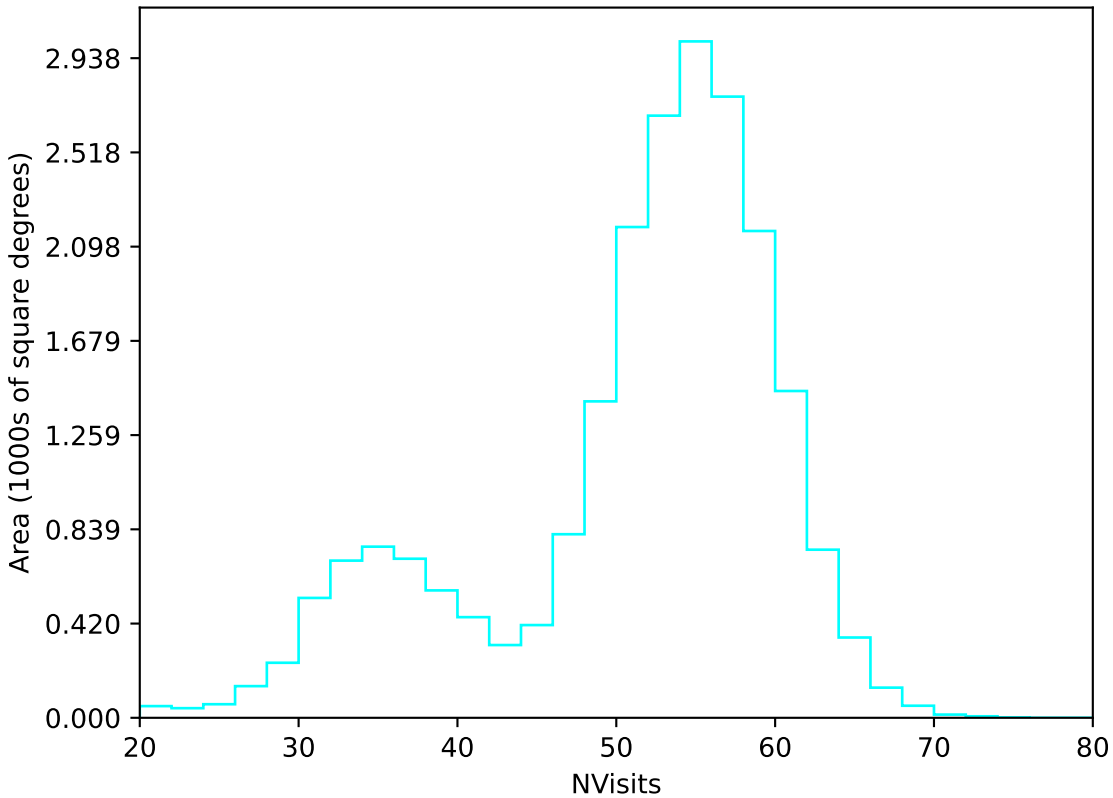
retro_baseline_v2.0_10yrs All sky u band: NVisits
