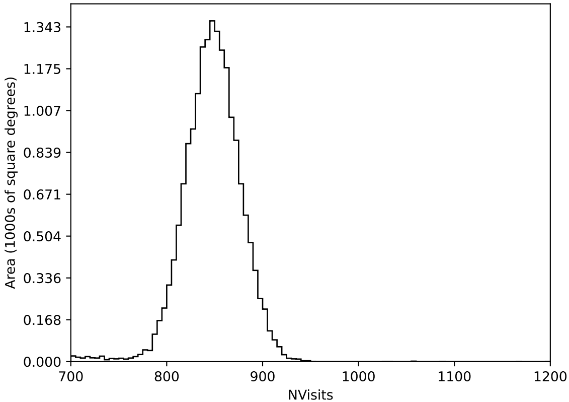
retro_baseline_v2.0_10yrs All sky all bands: NVisits
