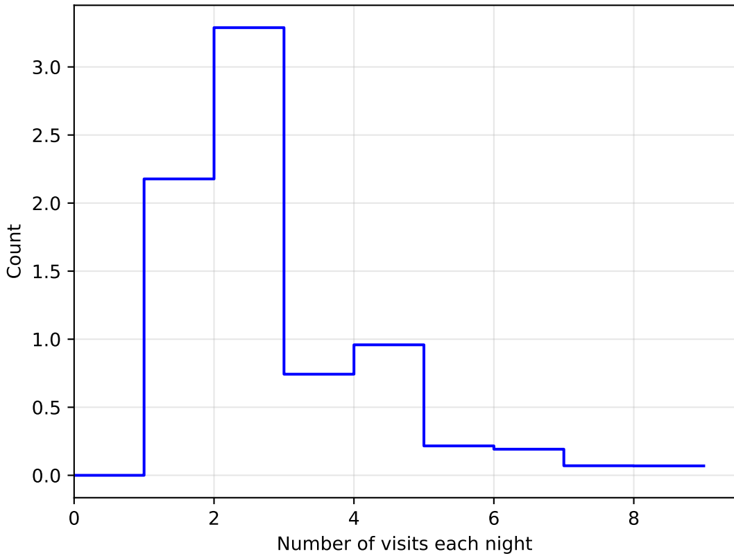
1e6 retro_baseline_v2.0_10yrs WFD: NVisitsPerNight
