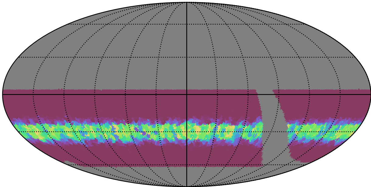
retro_baseline_v2.0_10yrs WFD u band: Min normairmass
