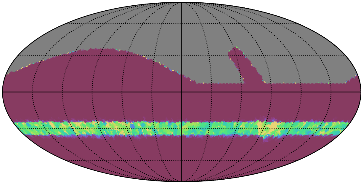
retro_baseline_v2.0_10yrs All sky all bands: Min normairmass
