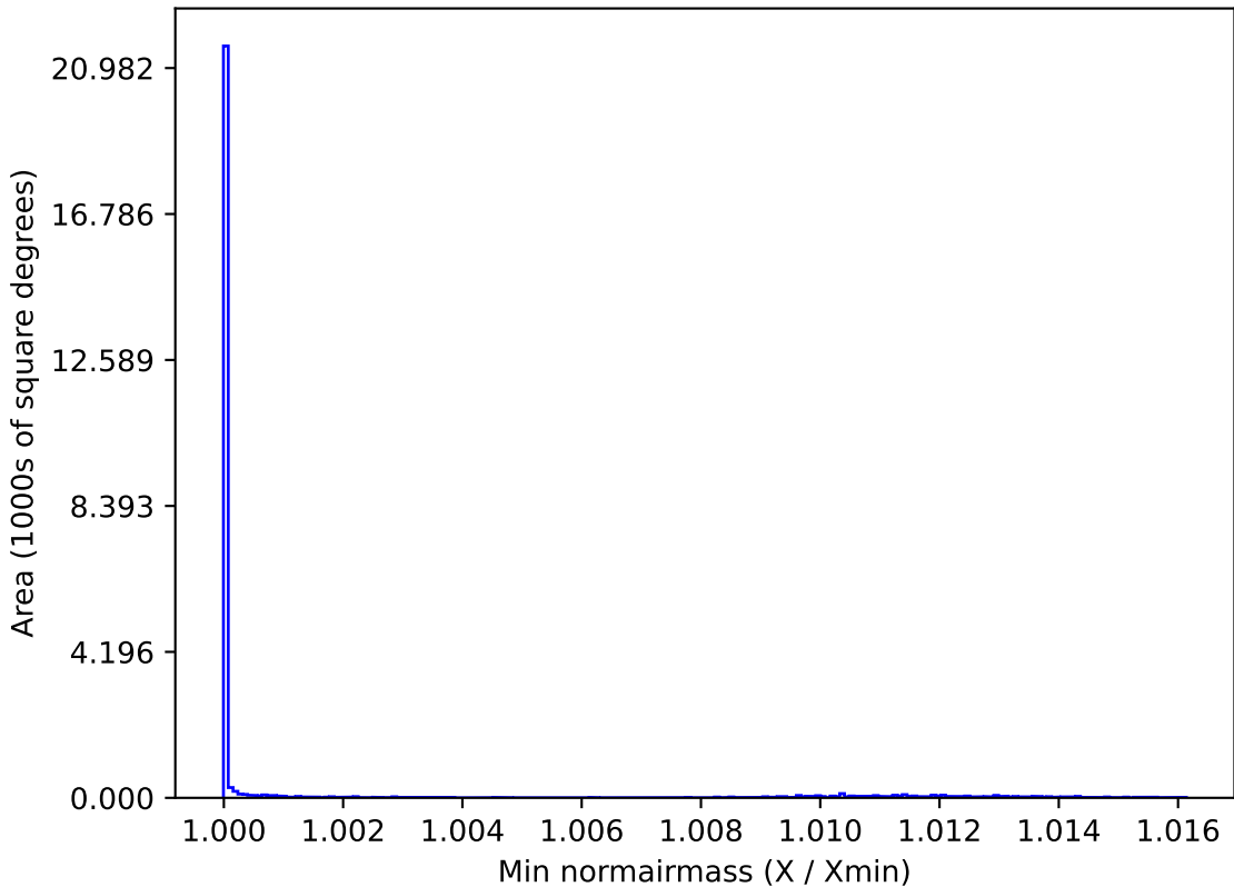
retro_baseline_v2.0_10yrs All sky all bands: Min normairmass
